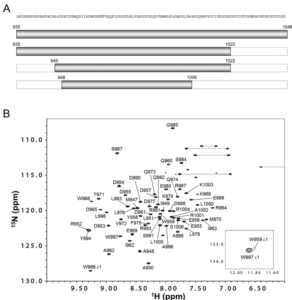
Fig. 1. PSV VPg protein constructs (A) and ^1\text{H} - ^{15}\text{N} HSQC spectrum of PSV VPg C (Ala948–Ser1006) (B). Residue numbers are labeled on the cross peaks. Cross peaks from the two tryptophan side chains of PSV VPg are shown in the inset.
